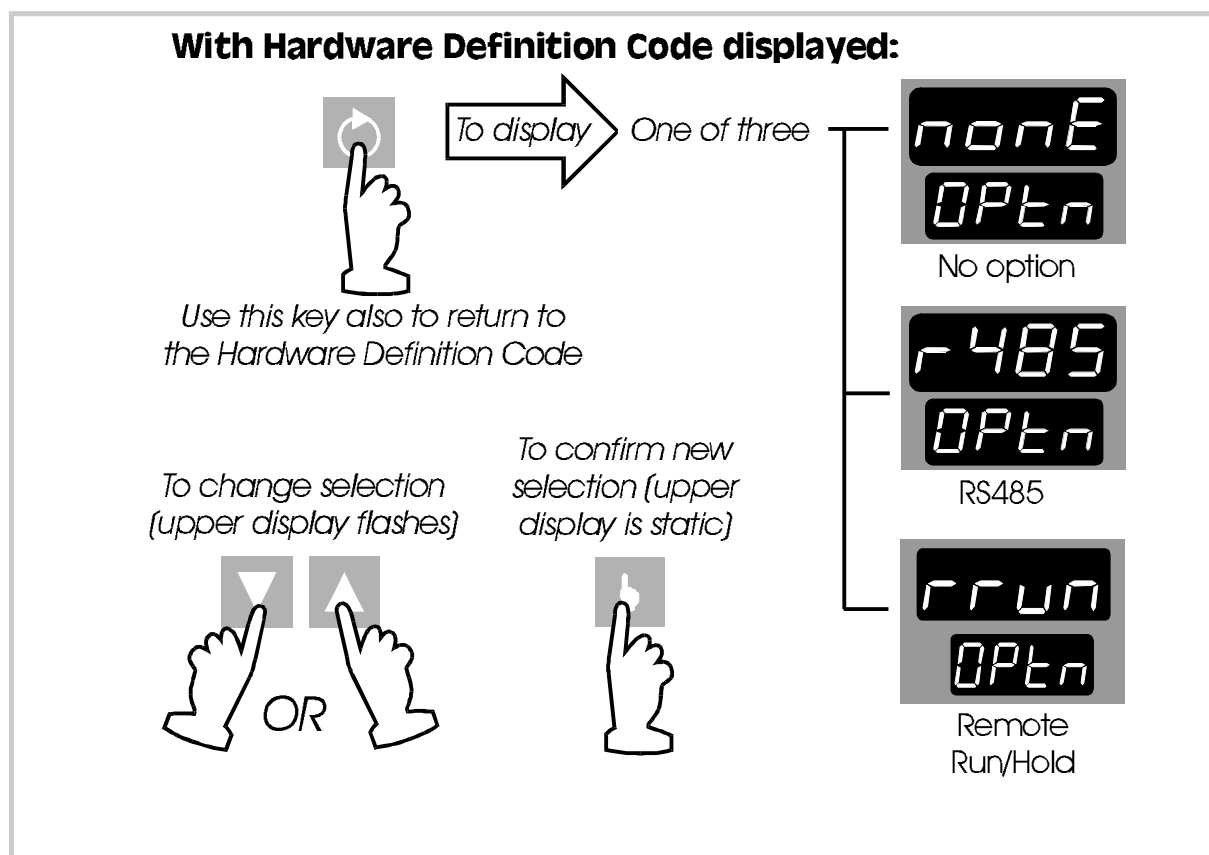
Figure 3-3 Option Selection
