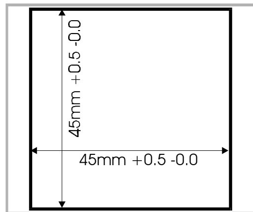
Figure 1-1 Cut-out Dimensions
