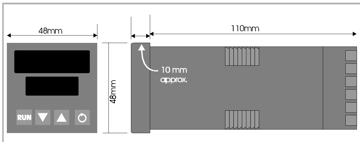
Figure 1-2 Main Dimensions
